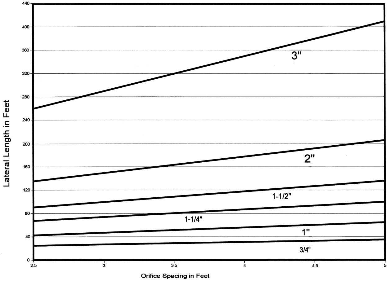
Minimum Lateral Diameter Based on Orifice Spacing for 5/32" Diameter Orifices
