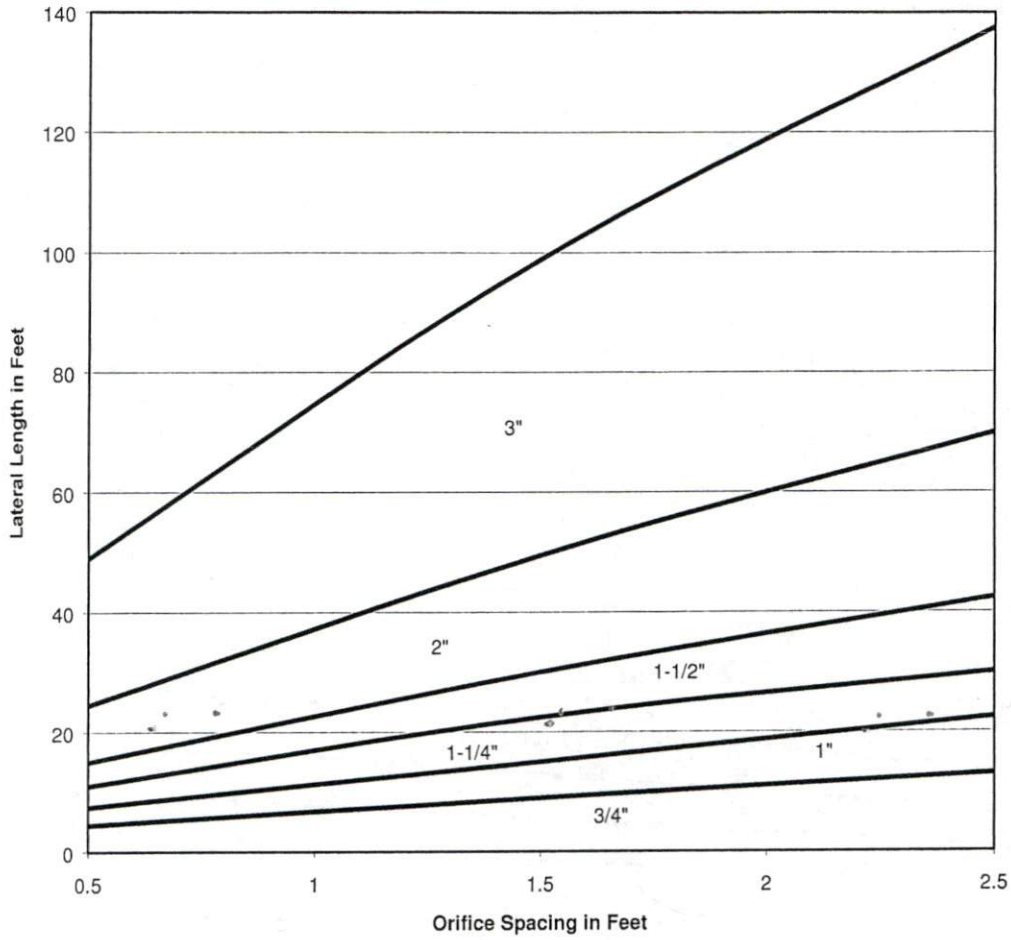
Minimum Lateral Diameter Based on Orifice Spacing for 1/4" Diameter Orifices
