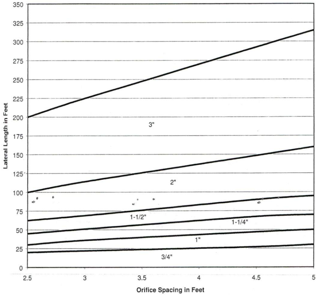
Minimum Lateral Diameter Based on Orifice Spacing for 3/16" Diameter Orifices
