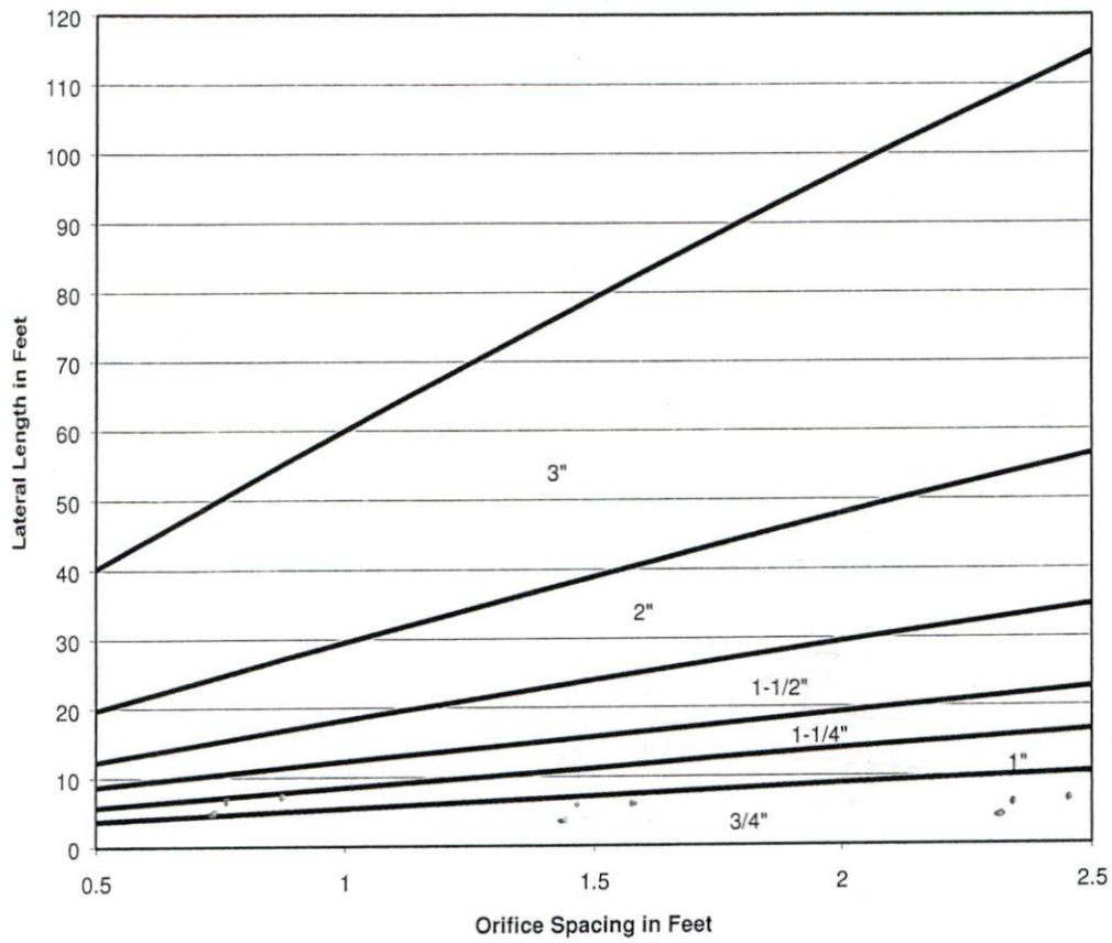
Minimum Lateral Diameter Based on Orifice Spacing for 5/32" Diameter Orifices
