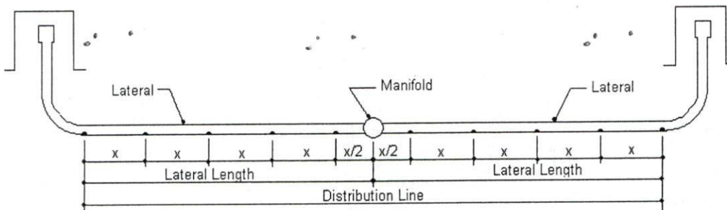
Figure 3 – Number of Orifices in a Distribution Line
